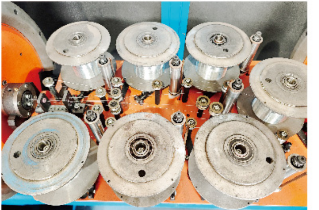
内放外收放线架 Inner pay-off cradle
