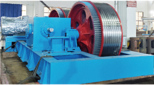
牵引轮 Traction capstan
