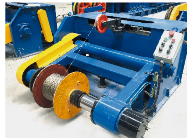
气动收线架 Pneumatic Take-off Stand
