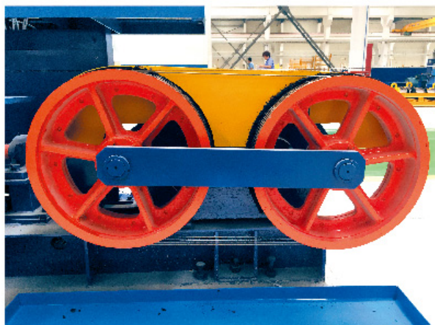
牵引轮 Dual wheel capstan
