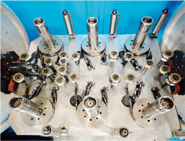
内放外收放线架 Inner pay-off cradle
